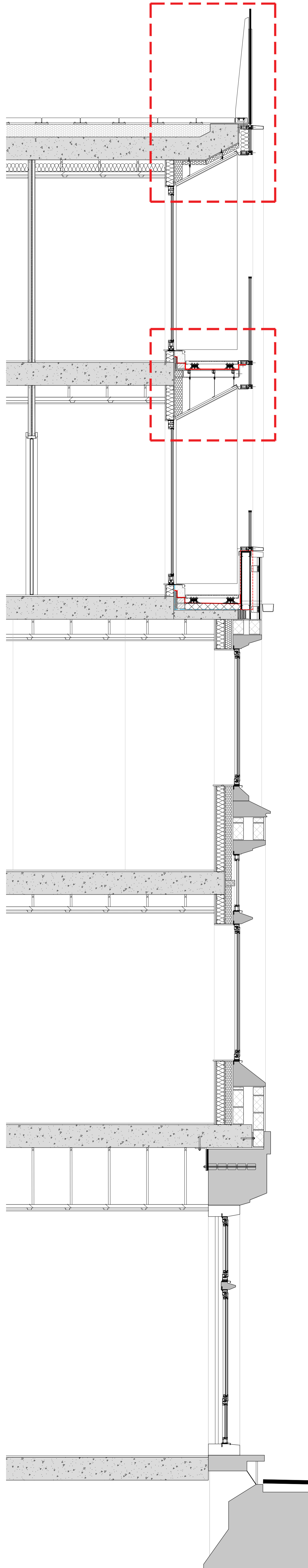
Section Key 1:25
