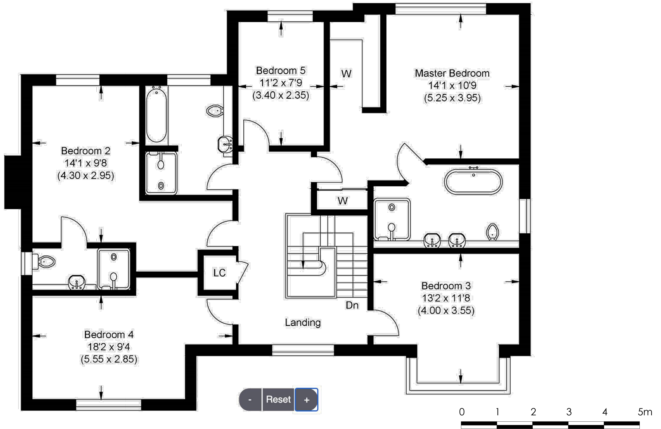
Existing First Floor Plan - Drawing No. 230316-07
