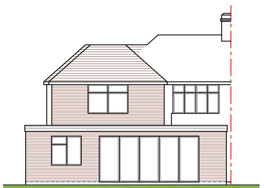
PROPOSED REAR ELEVATION 1:100@A3
