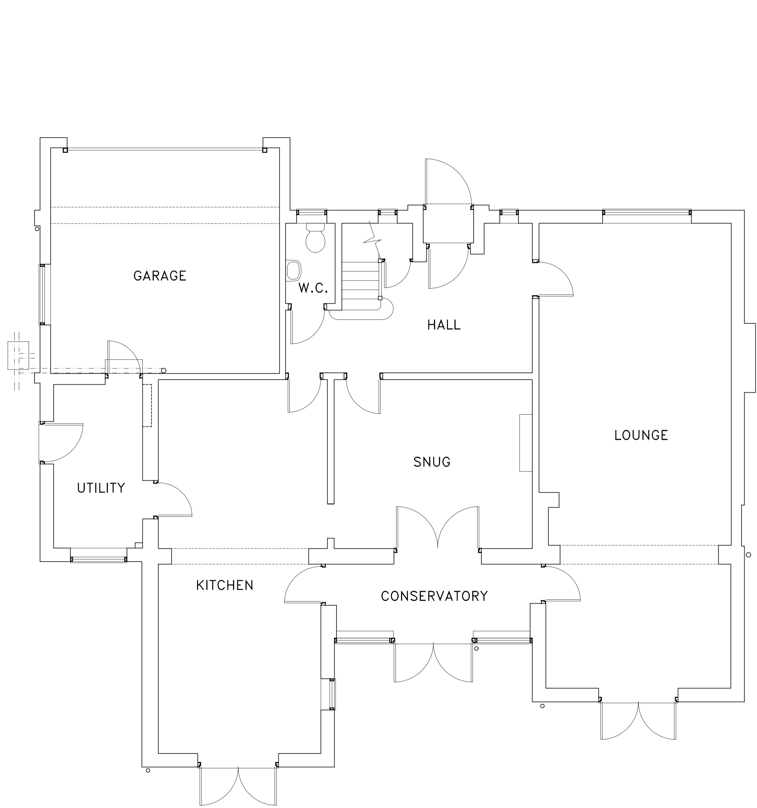
EXISTING GROUND FLOOR PLAN 1:50
