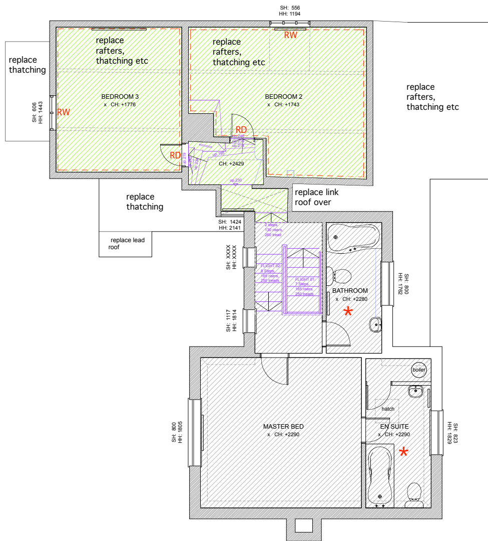
FIRST FLOOR INTERNAL FLOOR AREA : 73 SQ.M
