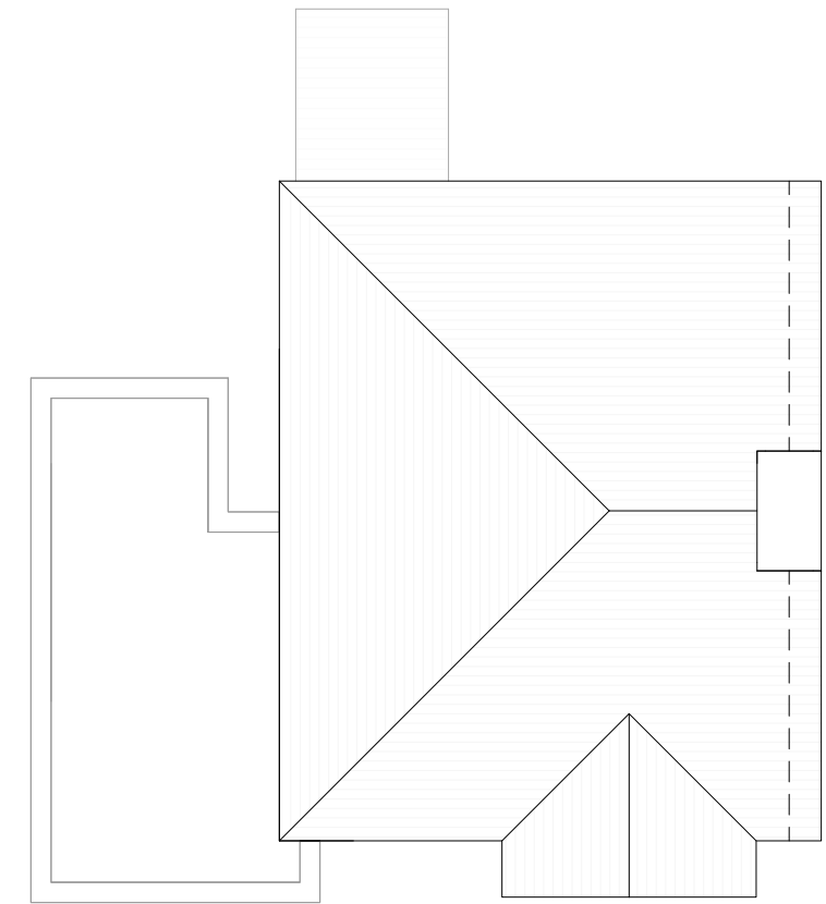
Roof Plan
