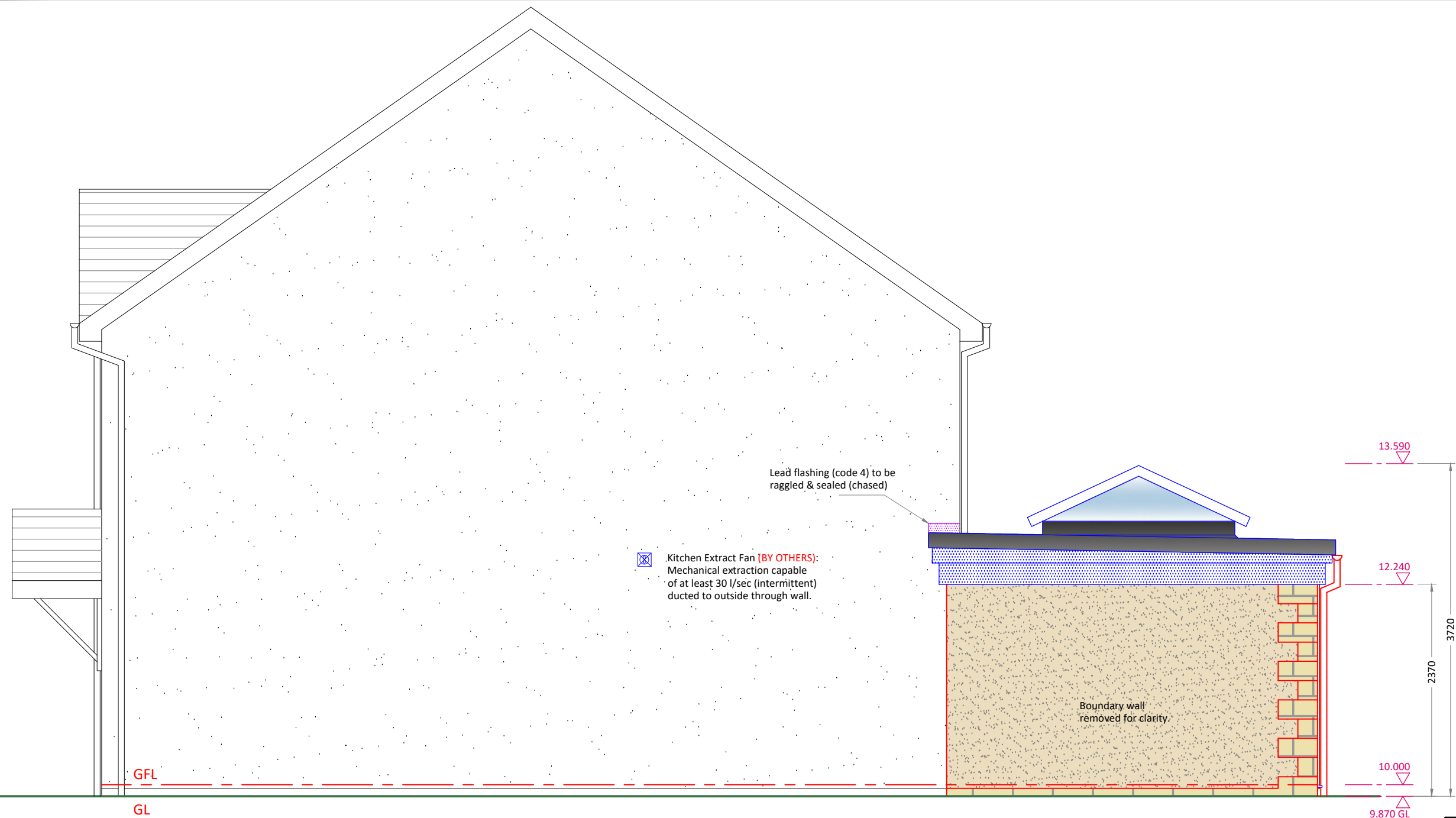
Proposed North - West Elevation (1:50)
