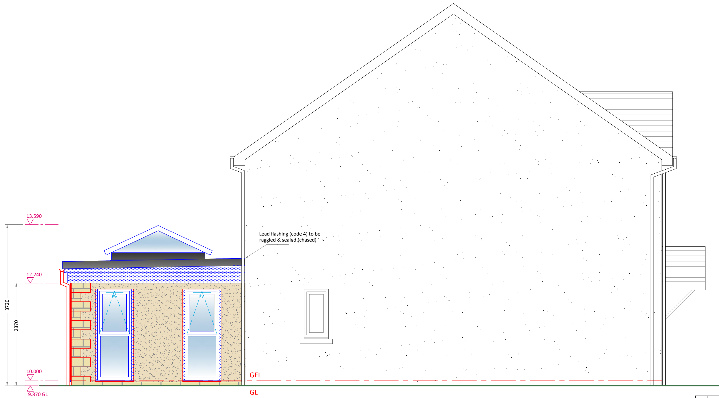
Proposed South - East Elevation (1:50)
