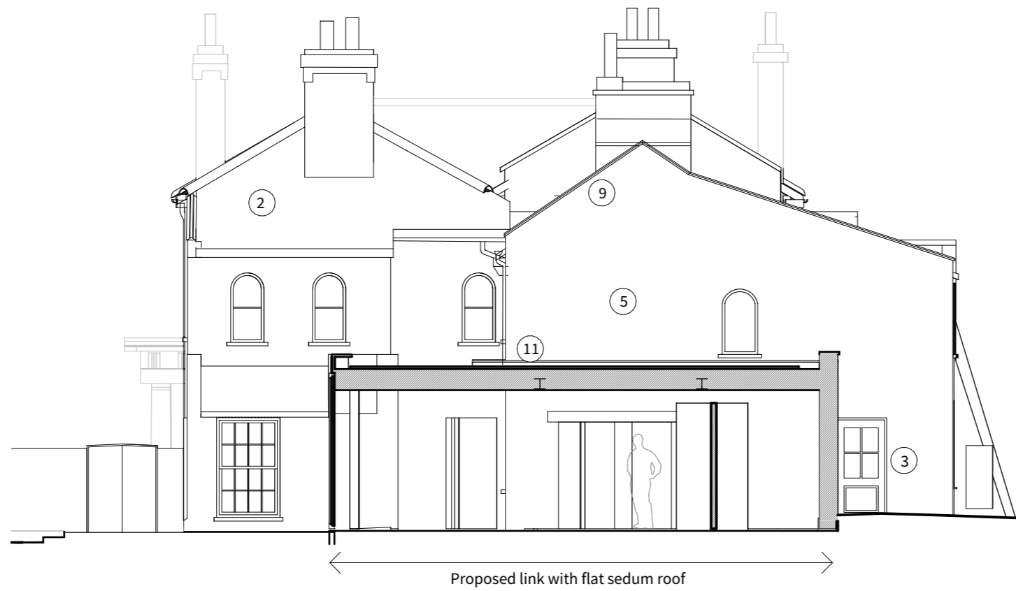
North Elevation (N1)
