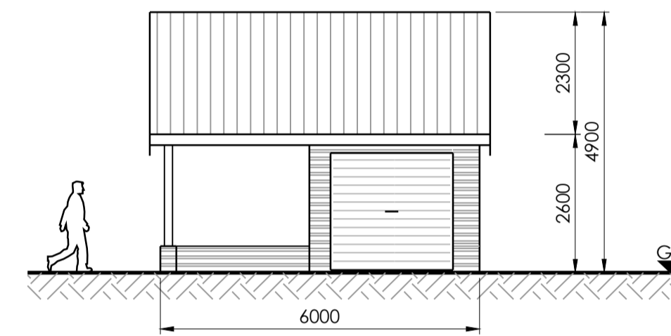
Front Elevation
