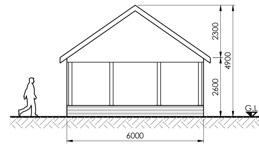
Side Elevation
