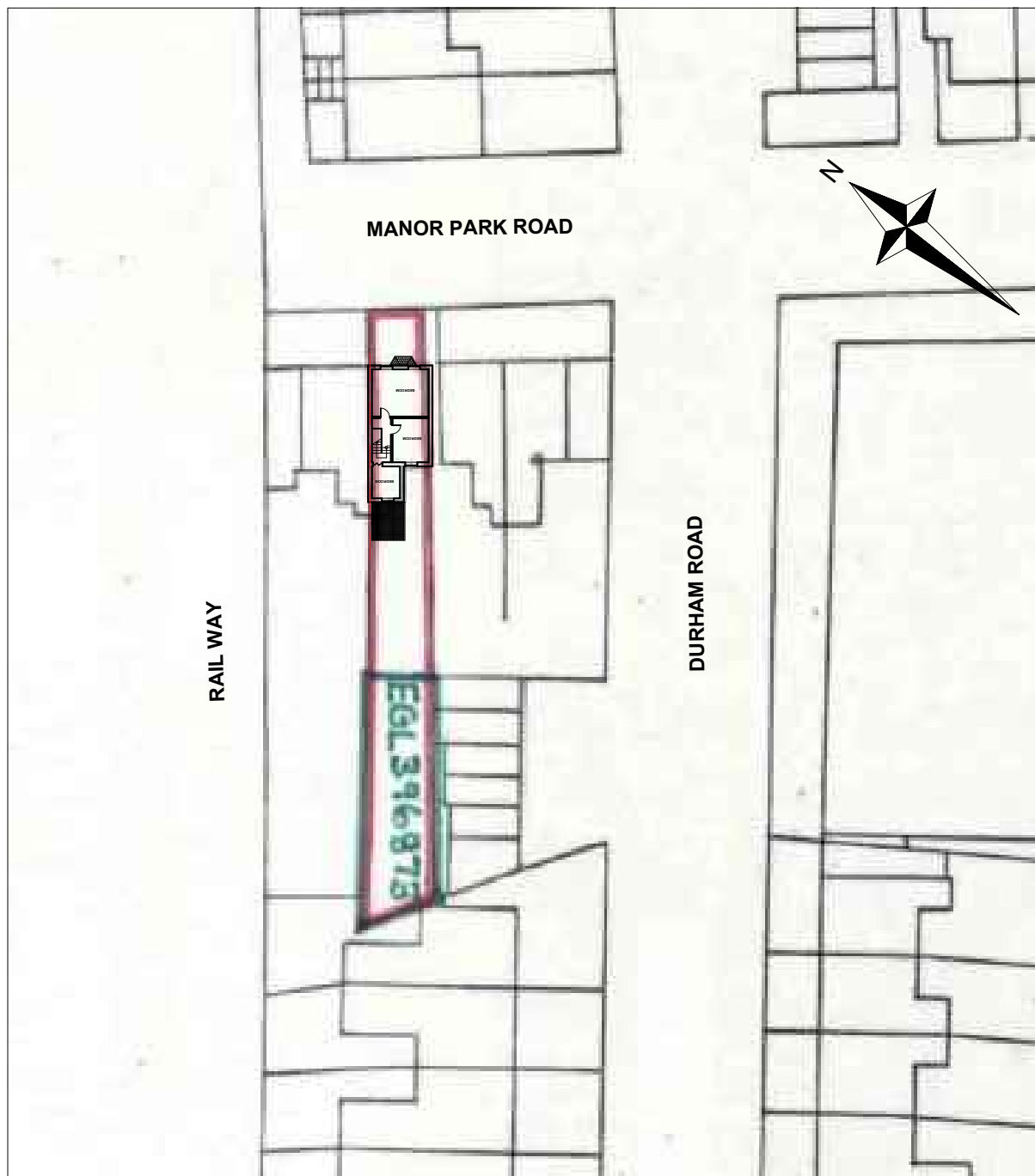
PRE-EXISTING BLOCK PLAN SCALE-1:500
