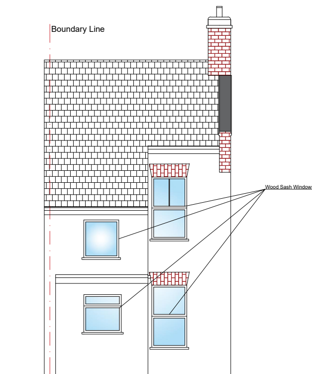
PRE-EXISTING REAR ELEVATION
