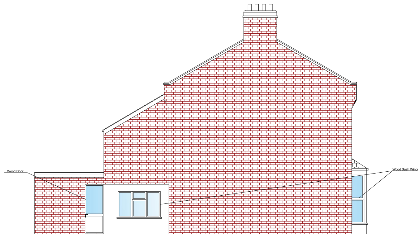
PRE-EXISTING LEFT SIDE ELEVATION
