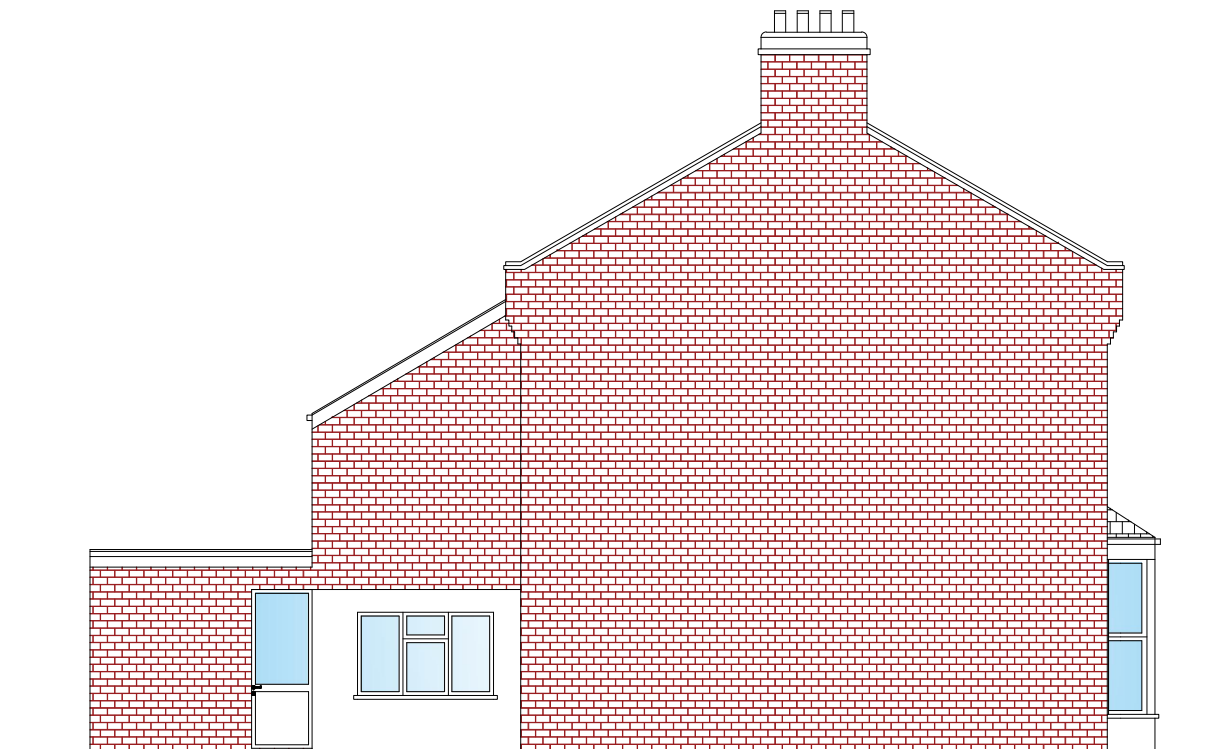
PRE-EXISTING LEFT SIDE ELEVATION
