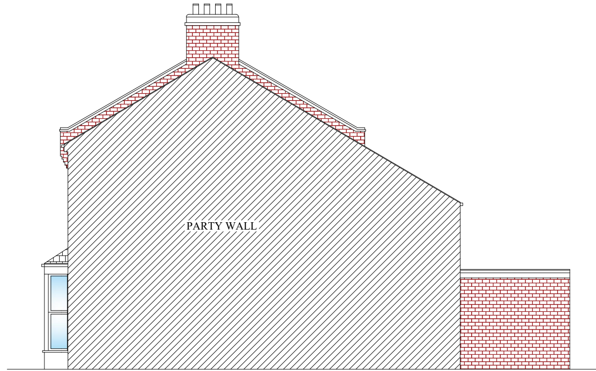
PRE-EXISTING RIGHT SIDE ELEVATION
