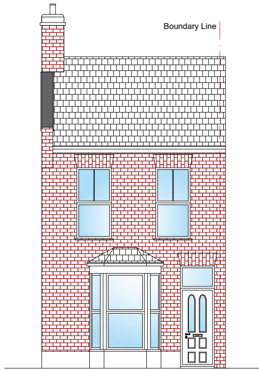
PRE-EXISTING FRONT ELEVATION
