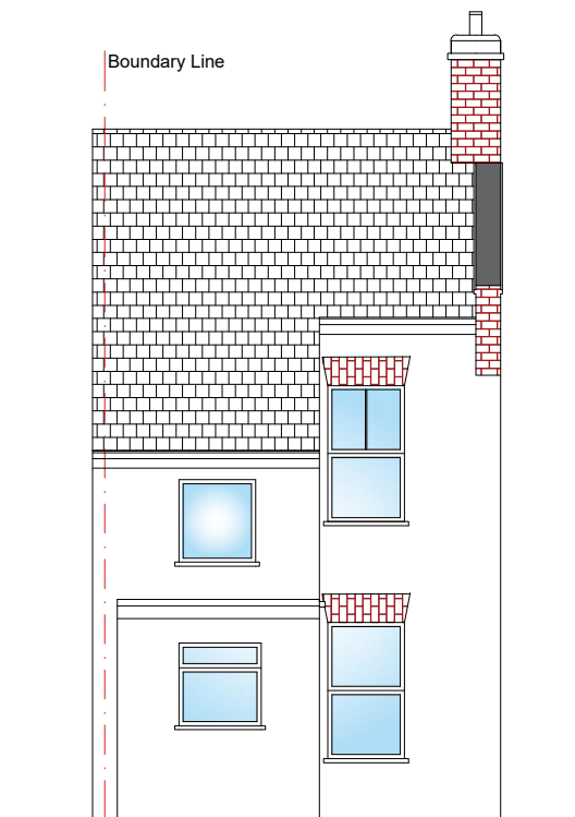
PRE-EXISTING REAR ELEVATION
