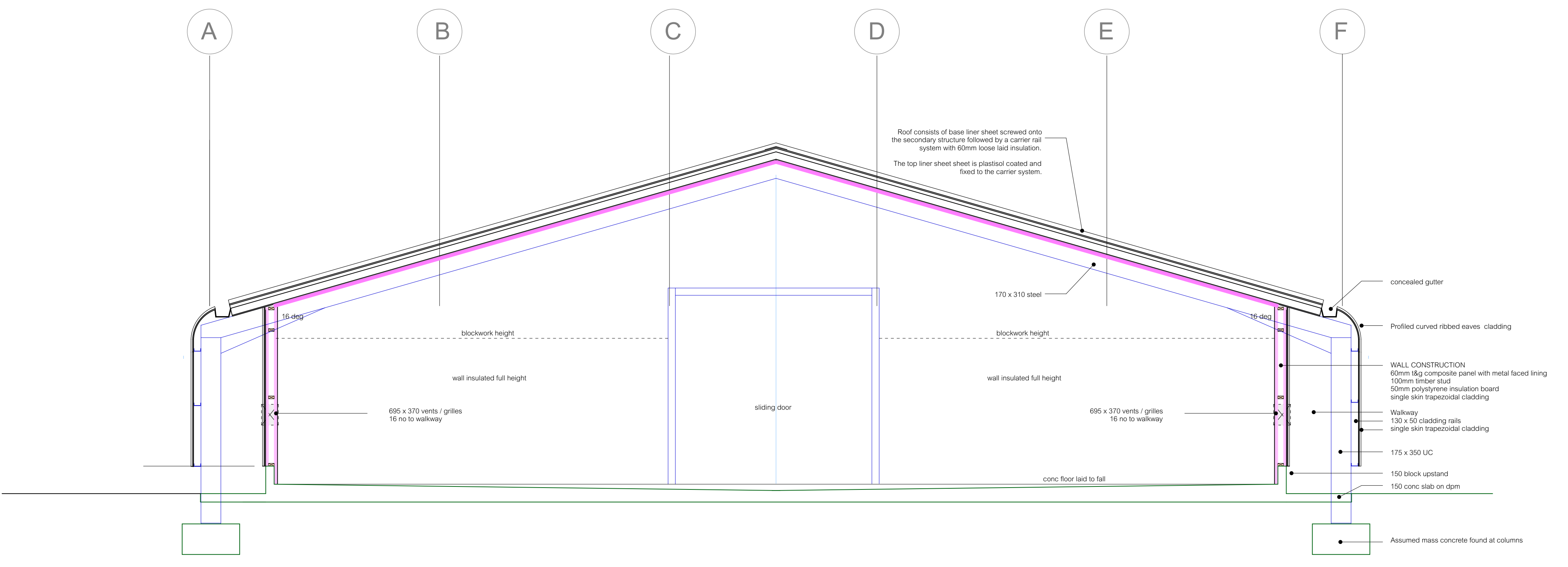
SECTION B-B
