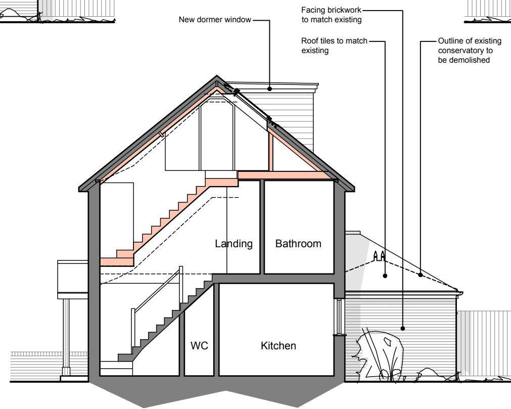
Section
