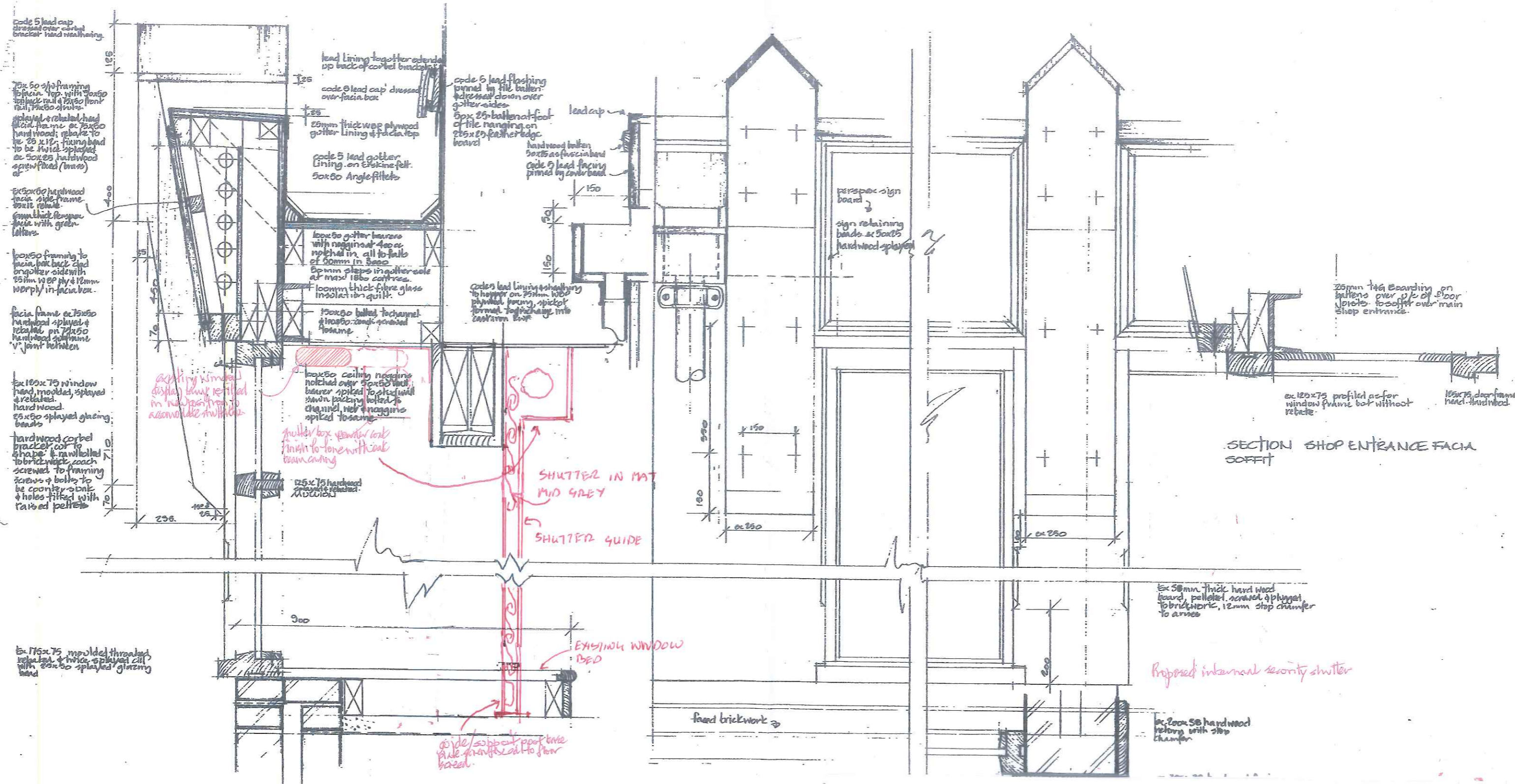
TYPICAL SECTION THROUGH SHOP FRONT & FACIA.
