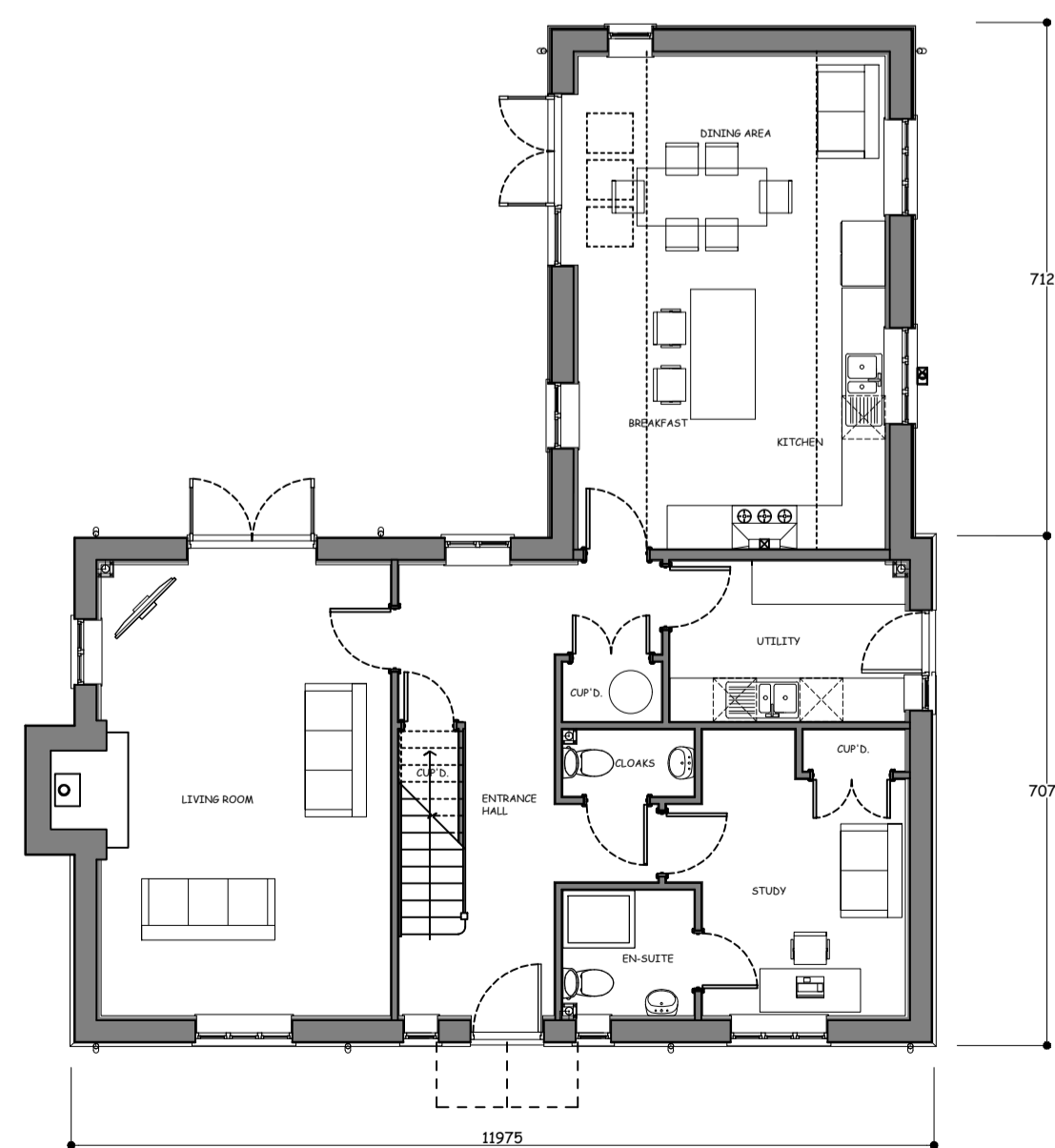
GROUND FLOOR PLAN - 1/100 scale PLOT no 3
