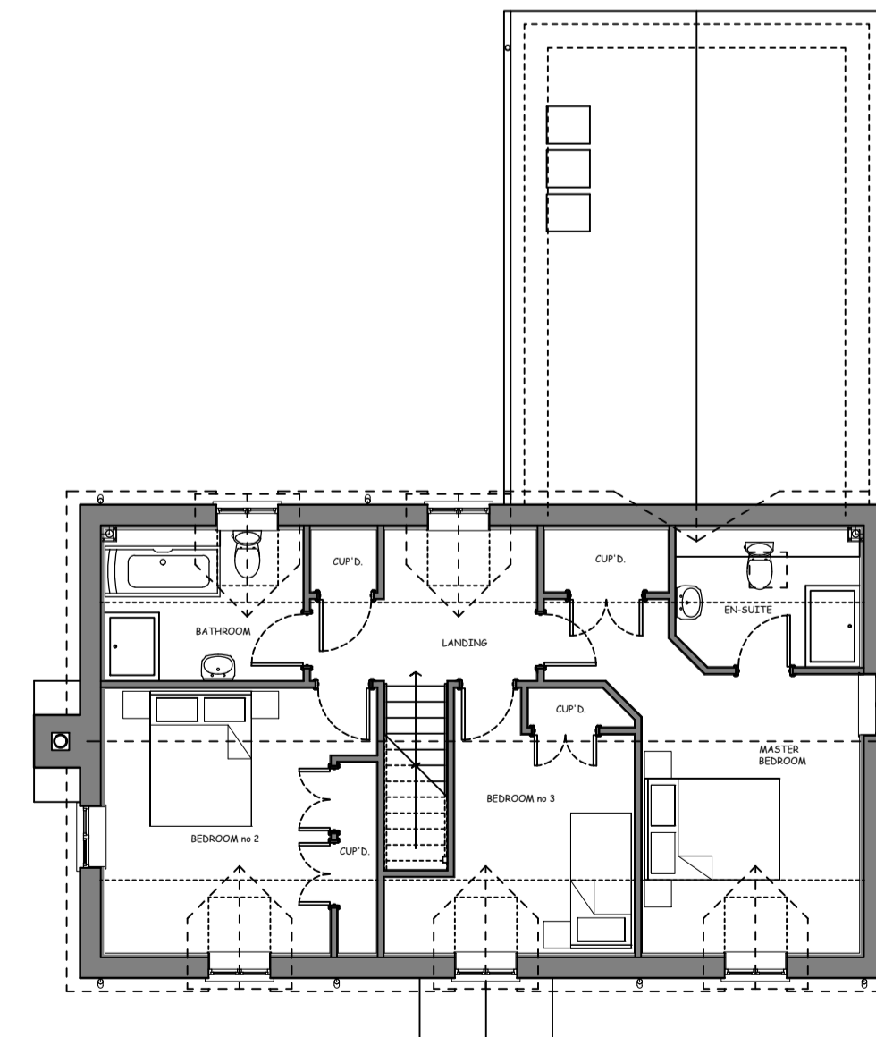
FIRST FLOOR PLAN - 1/100 scale PLOT no 3
