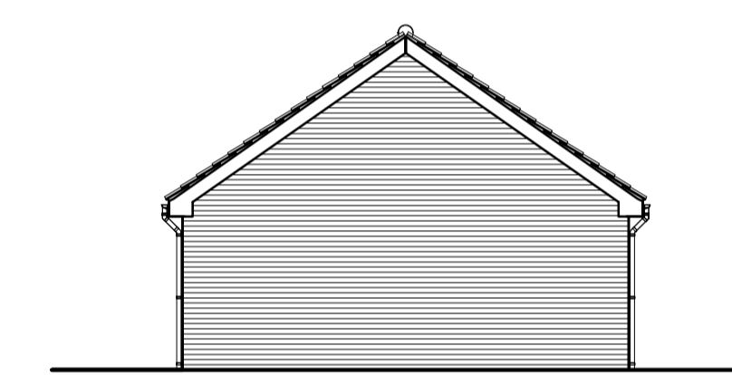
NORTH SIDE ELEVATION 1/100 scale. PLOT no 3.
