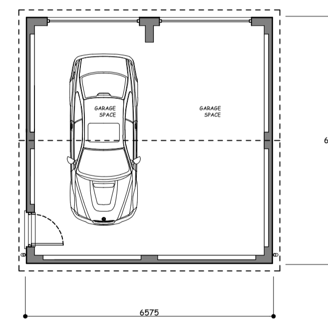
GROUND FLOOR PLAN GARAGE 1/100 scale. PLOT no 3
