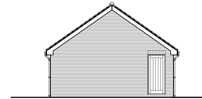
SOUTH SIDE ELEVATION 1/100 scale. PLOT no 3.
