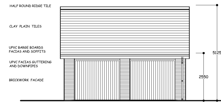
WEST FRONT ELEVATION 1/100 scale. PLOT no 3.
