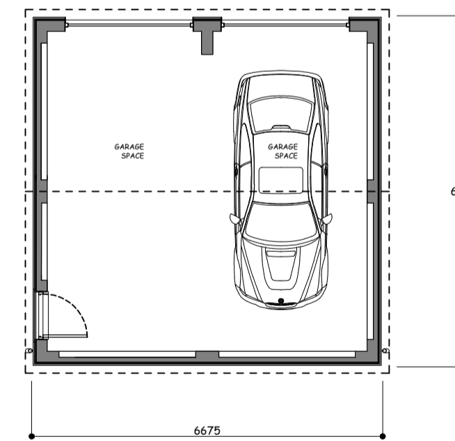
GROUND FLOOR PLAN GARAGE 1/100 scale. PLOT no 2
