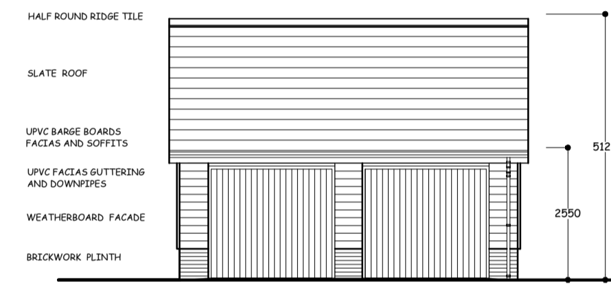
WEST FRONT ELEVATION 1/100 scale. PLOT no 2.
