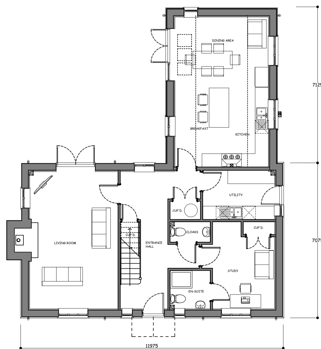
GROUND FLOOR PLAN - 1/100 scale PLOT no 2
