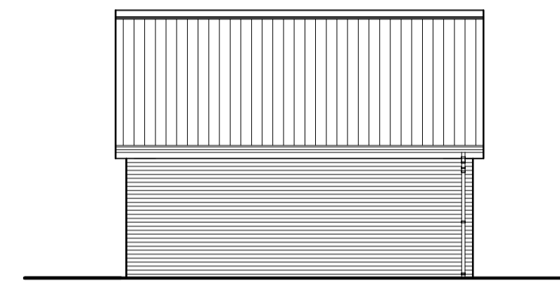
EAST REAR ELEVATION 1/100 scale. PLOT no 1.
