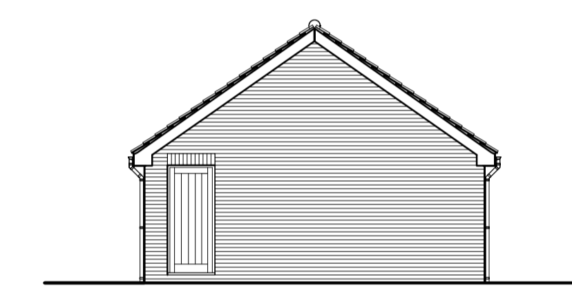
NORTH SIDE ELEVATION 1/100 scale. PLOT no 1.
