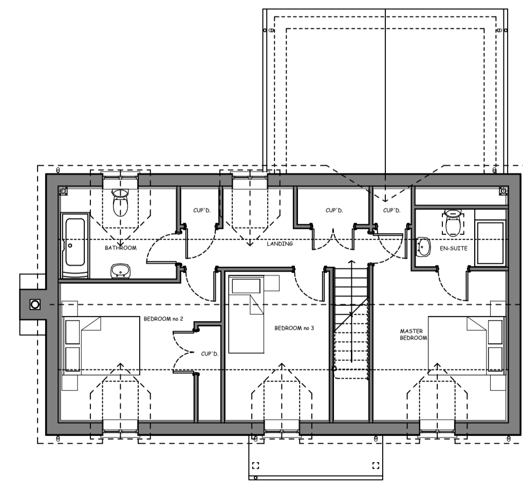
FIRST FLOOR PLAN - 1/100 scale PLOT no 1
