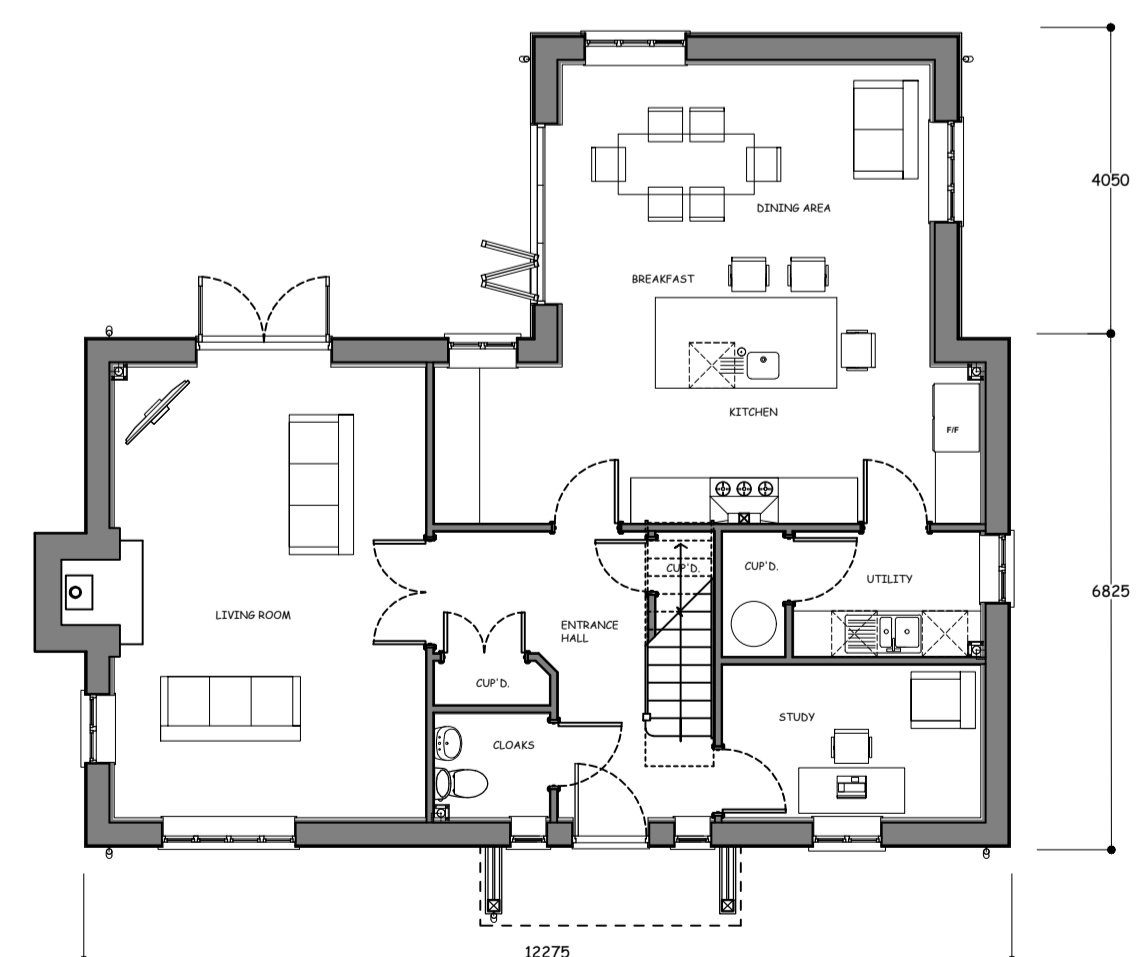
GROUND FLOOR PLAN - 1/100 scale PLOT no 1
