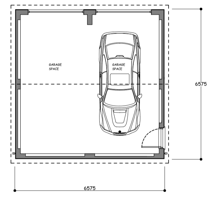
GROUND FLOOR PLAN GARAGE 1/100 scale. PLOT no 1.
