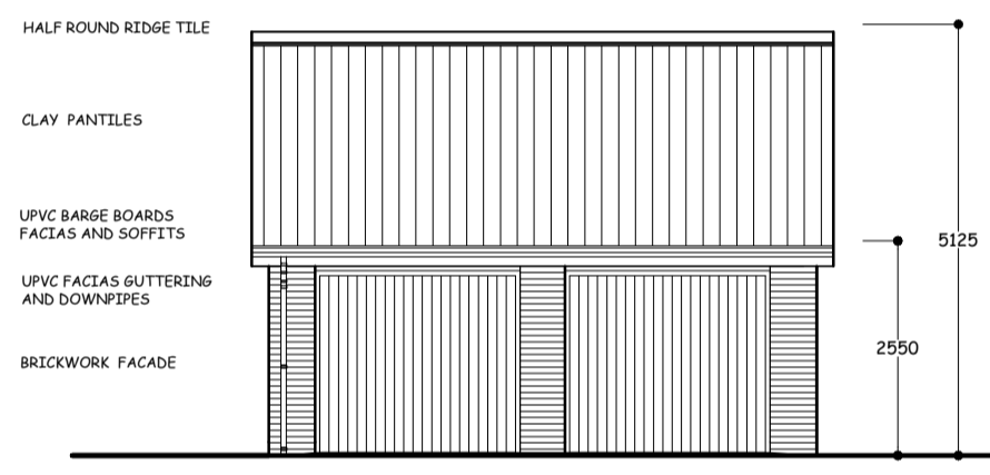
WEST FRONT ELEVATION 1/100 scale. PLOT no 1.
