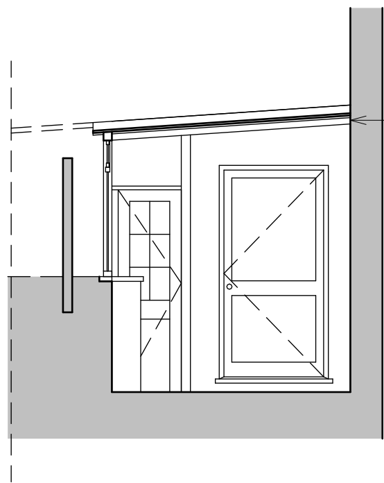
Short Section
