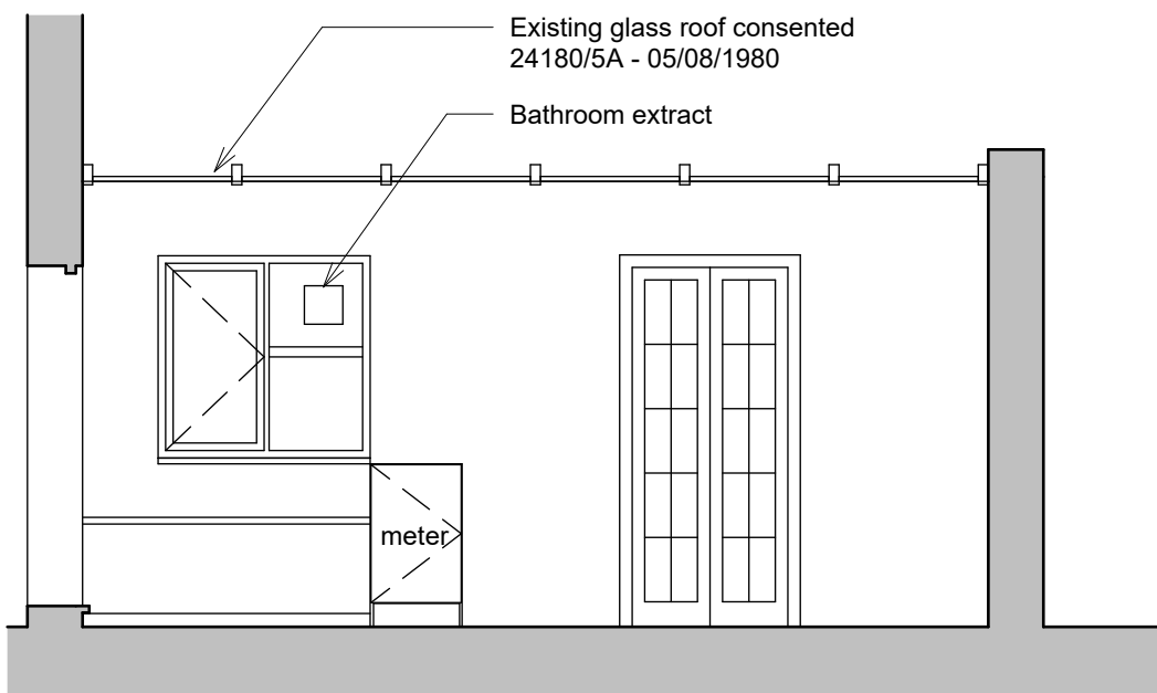
Long Section
