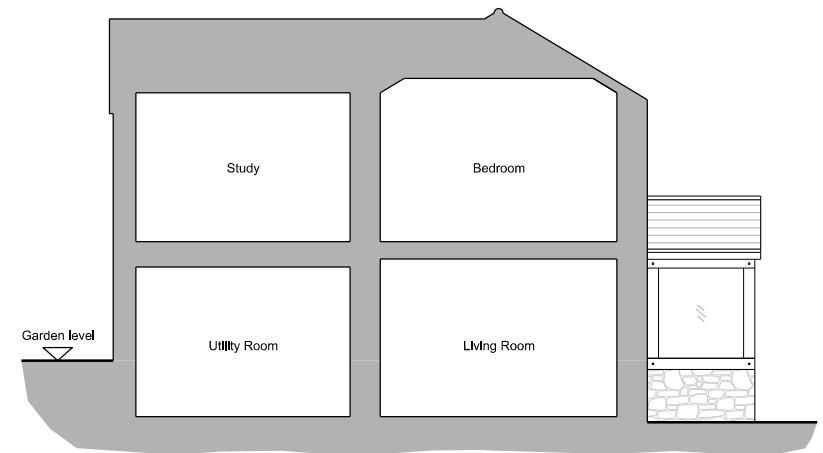
Proposed South Sectional Elevation
