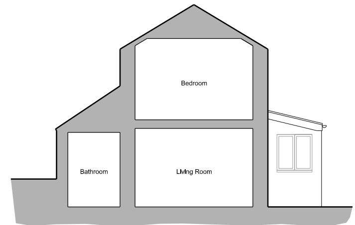
Existing South Sectional Elevation
