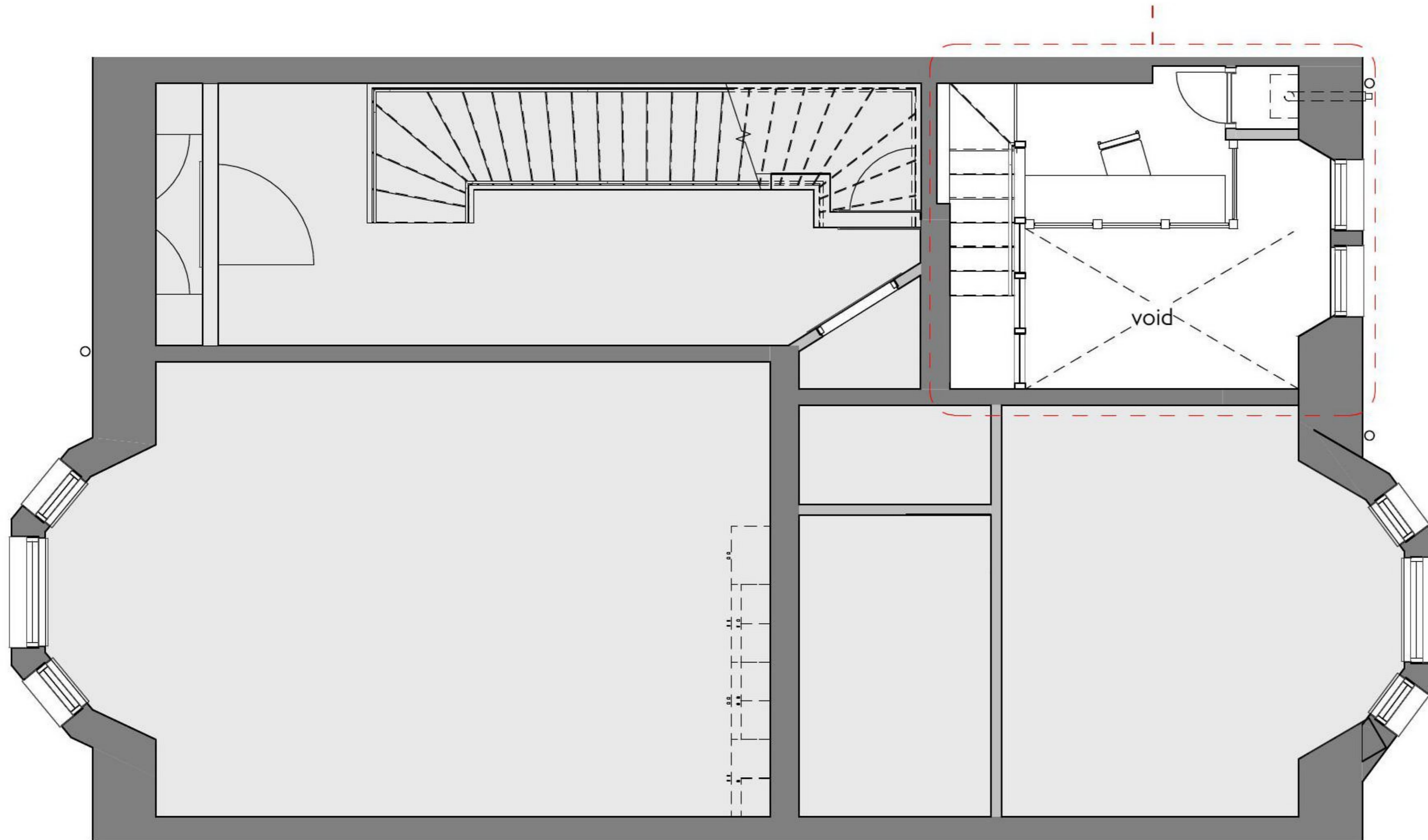
1 Proposed Mezzanine Plan 1 : 50
