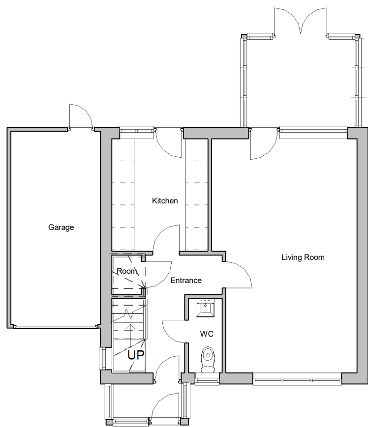
1 Ground Floor Plan 1 : 100
