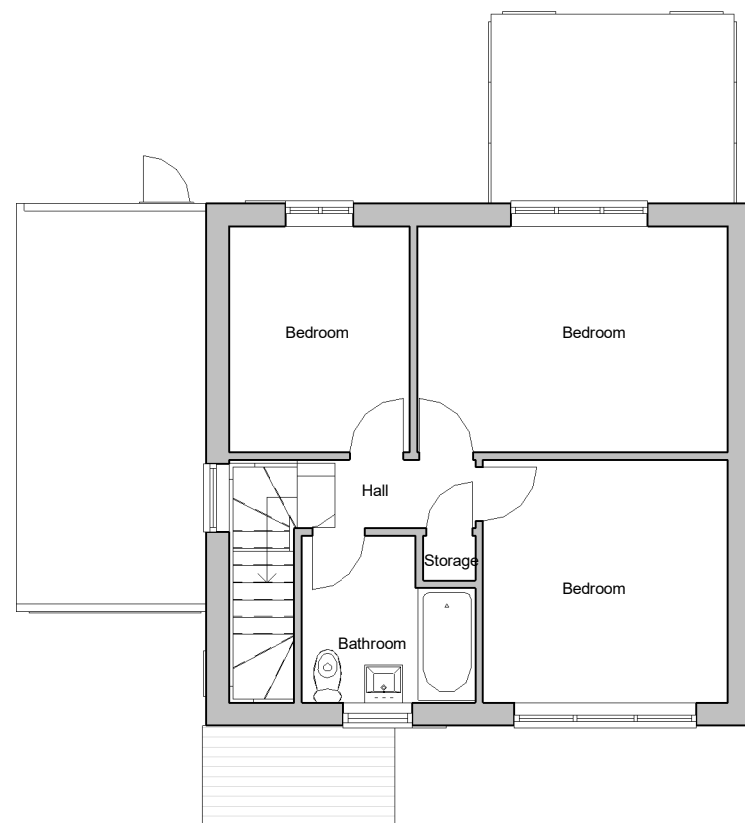
2 First Floor Plan 1 : 100
