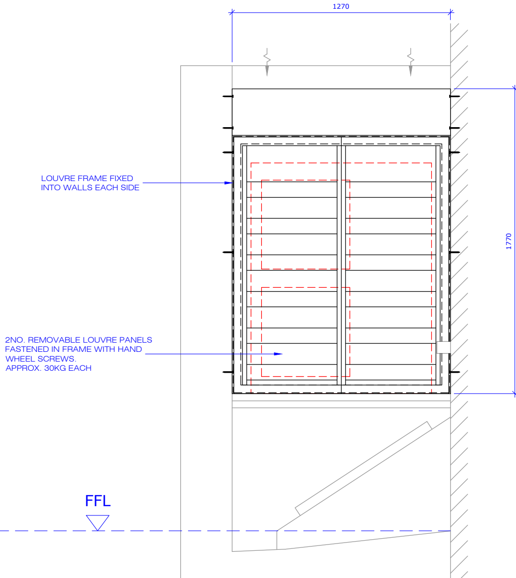
Front Elevation
