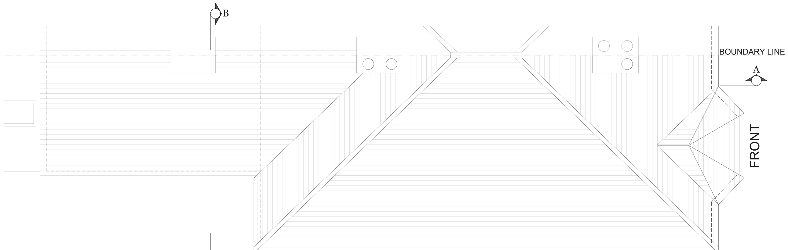
EXISTING ROOF TOP PLAN SCALE 1:50
