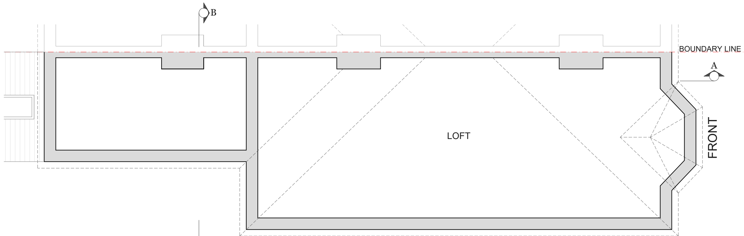
EXISTING LOFT FLOOR PLAN SCALE 1:50
