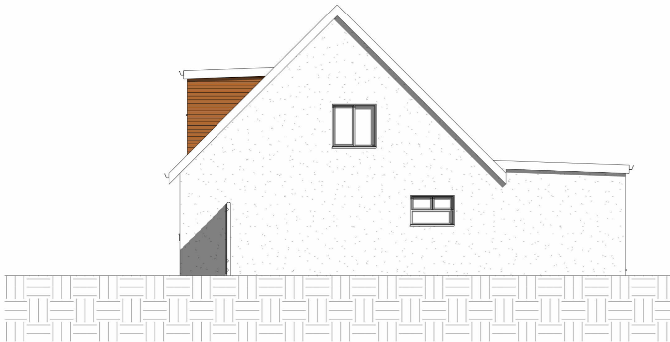
EXISTING SIDE ELEVATION (RHS) 1 : 100
