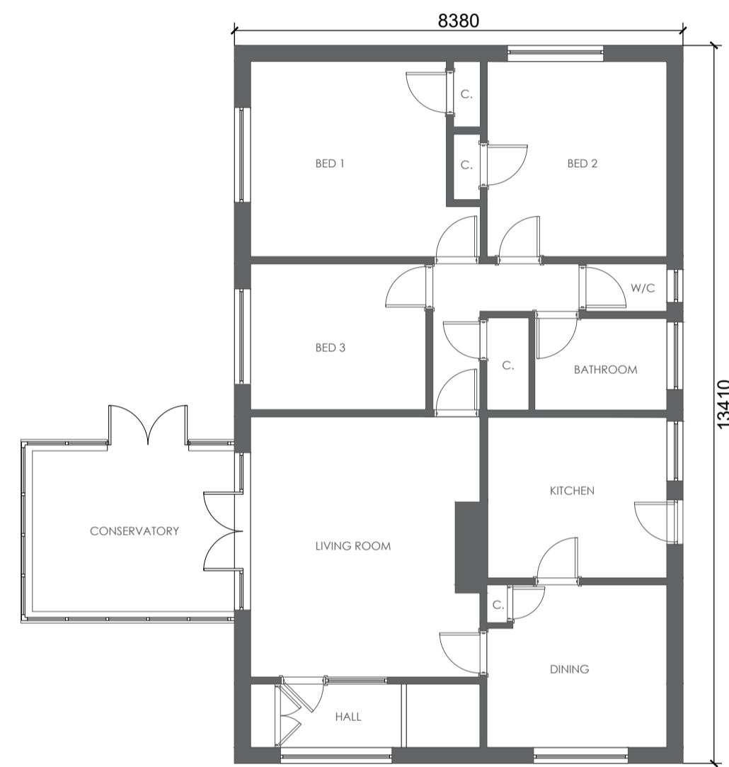
1:100 Ground Floor Plan
