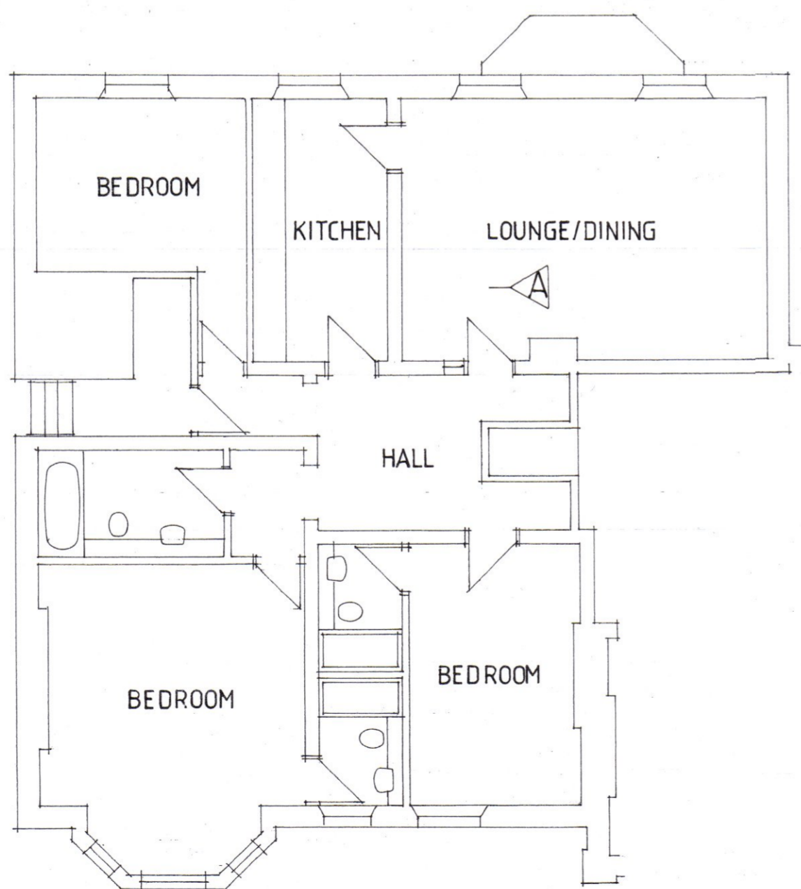
FIRST FLOOR PLAN as existing
