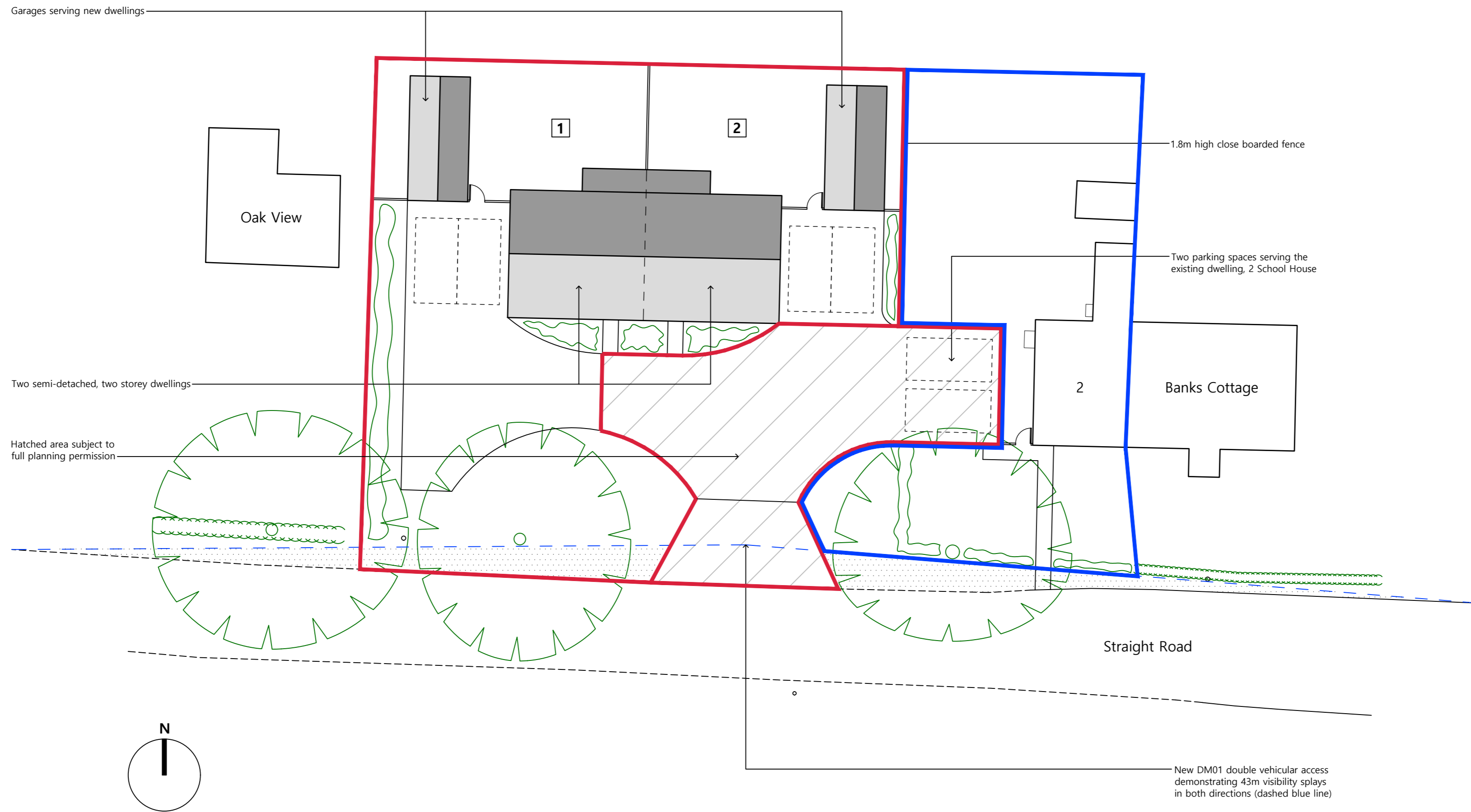
Proposed site plan 1:200
