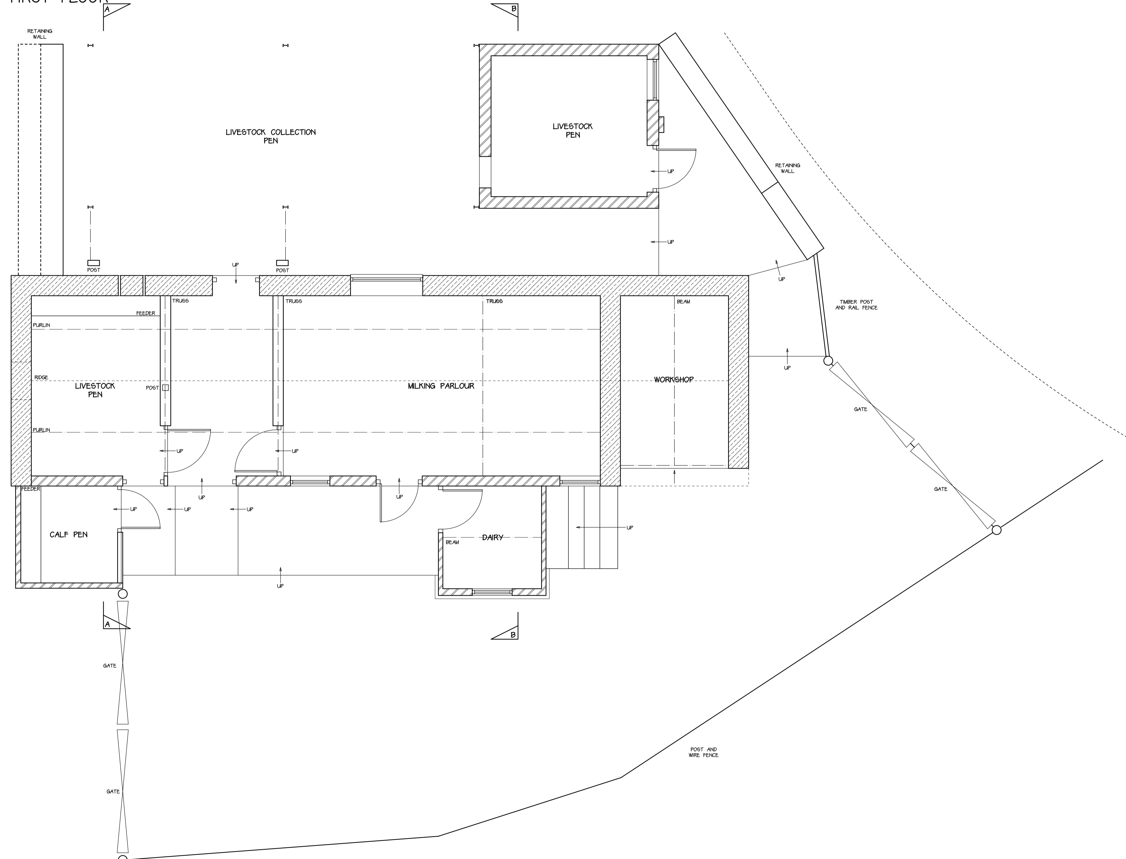
GROUND FLOOR EXISTING LAYOUTS 1 / 50
