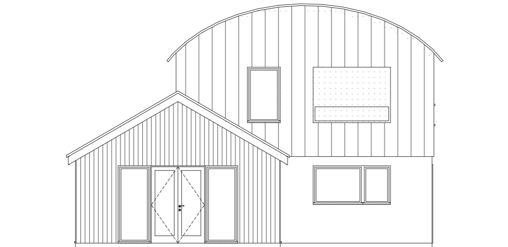
SOUTH ELEVATION
