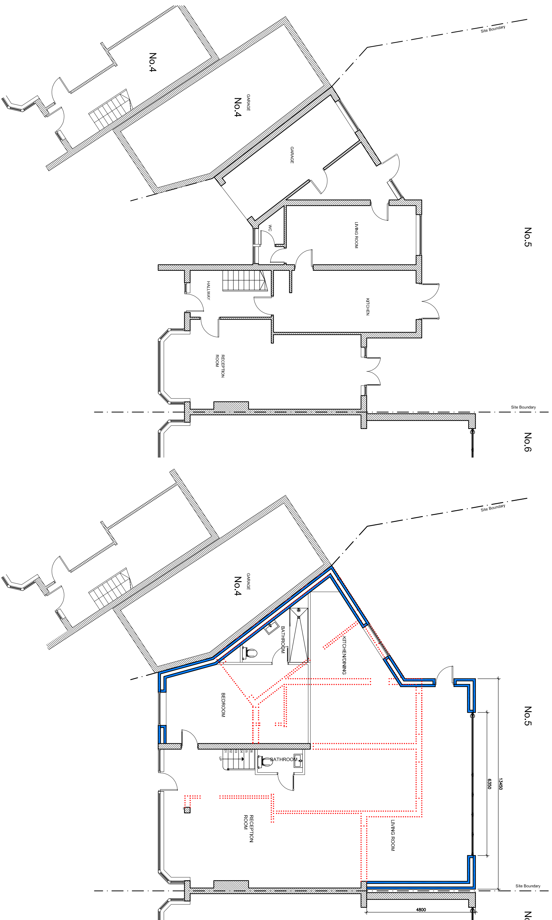
EXISTING GROUND FLOOR LAYOUT
