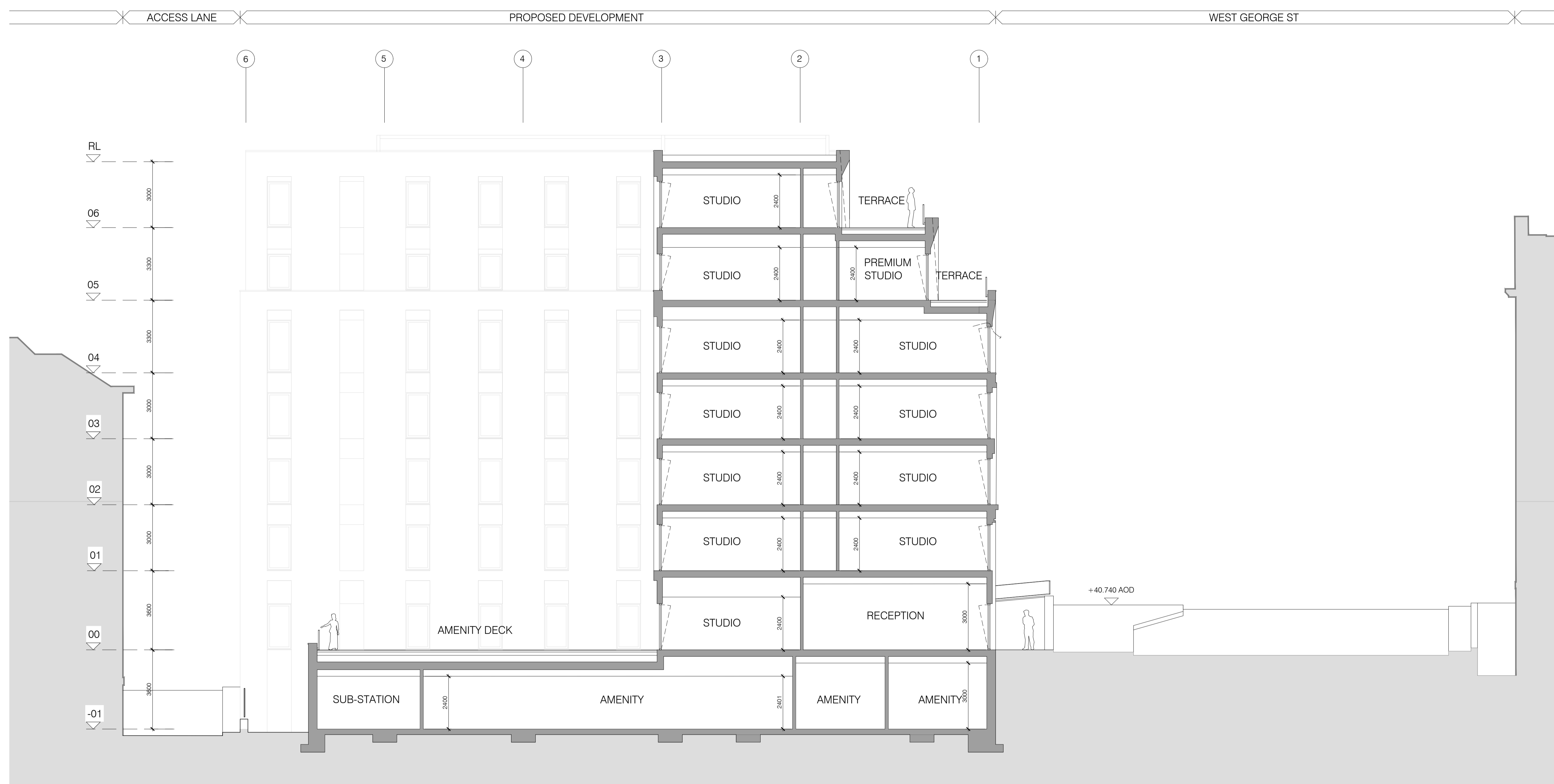
SECTION AA - AS PROPOSED
