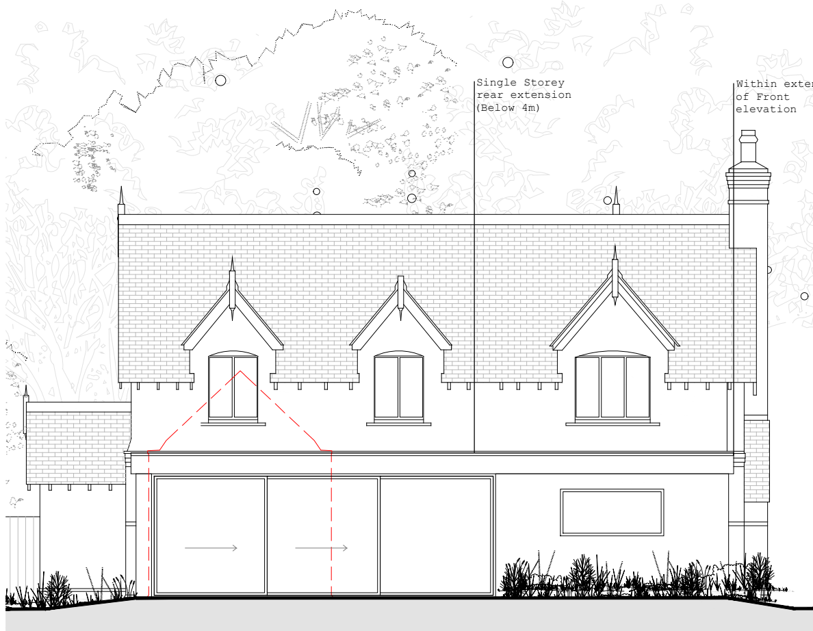
Proposed Rear Elevation (South)
