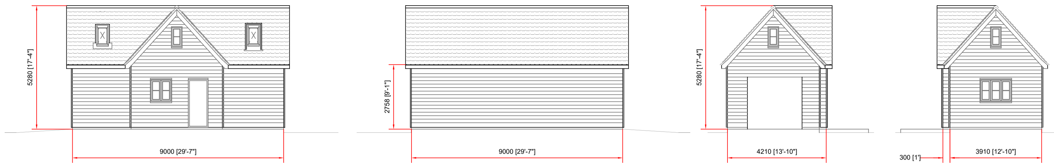
Existing Front Elevation Elevations 1:100 @ A1
