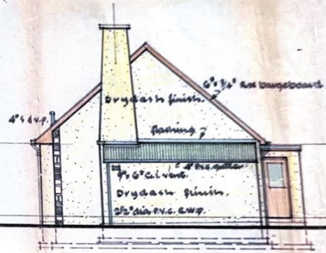
• WEST • ELEVATION •
