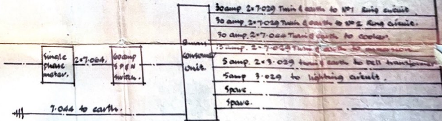
• ELECTRICAL SCHEMATIC DIAGRAM •
