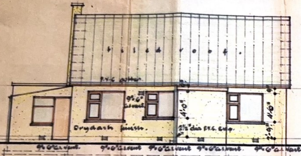
• SOUTH • ELEVATION •
