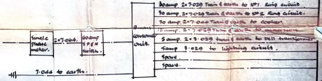
◦ ELECTRICAL SCHEMATIC DIAGRAM ◦
