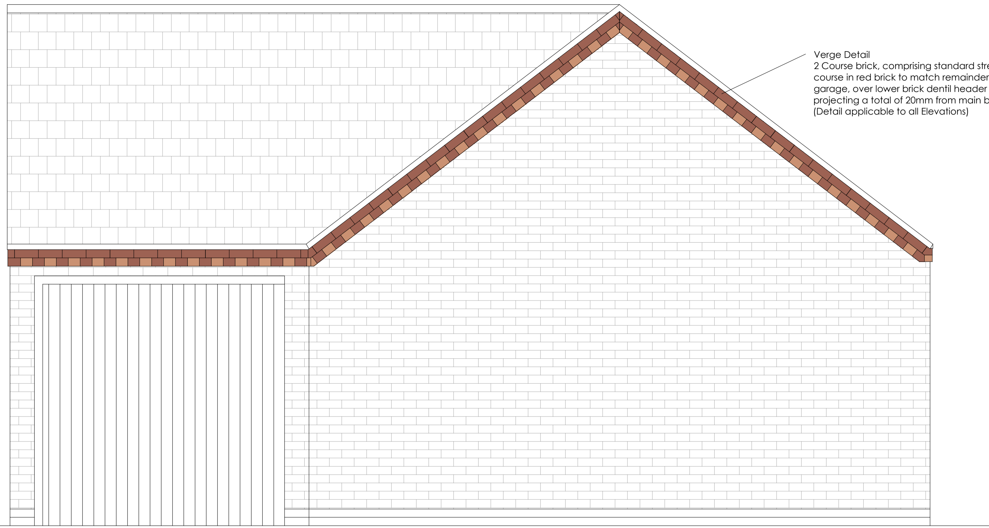
VERGE DETAIL- SCALE 1:20 - CONDITION 3
