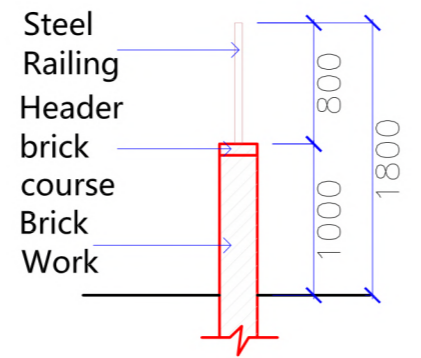
Proposed Section X-X
