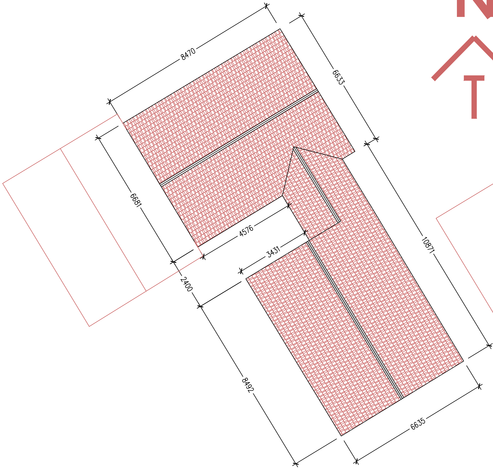
PROPOSED ROOF PLAN _OPTION C
