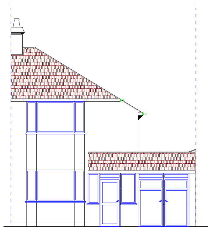
EXISTING REAR VIEW
