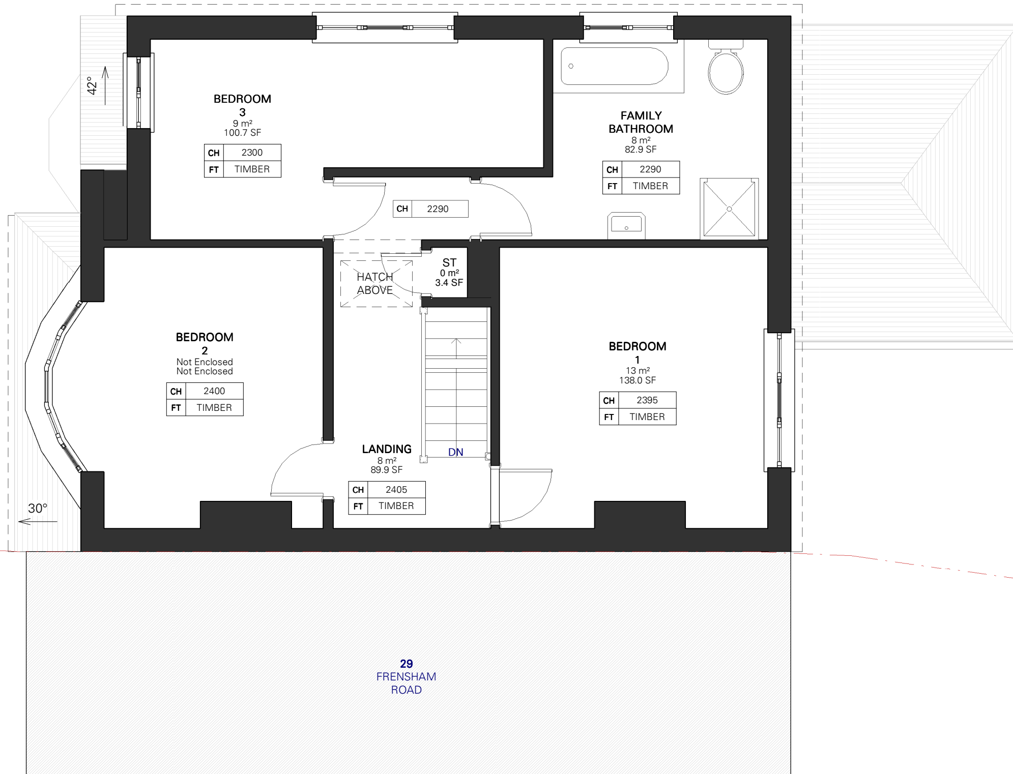
EXISTING FIRST FLOOR PLAN 1 : 50
