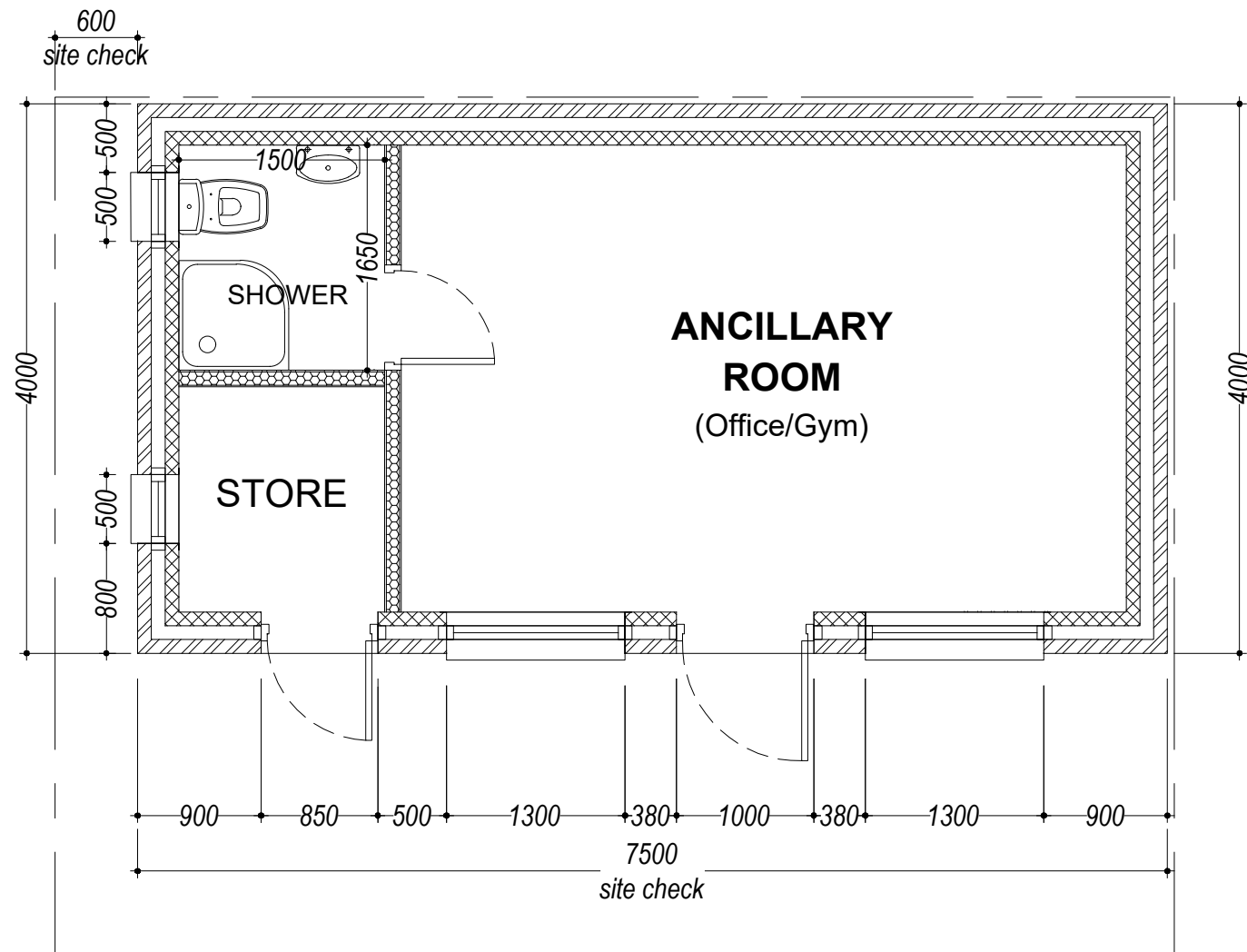
PROPOSED GROUND FLOOR PLAN 1:50
