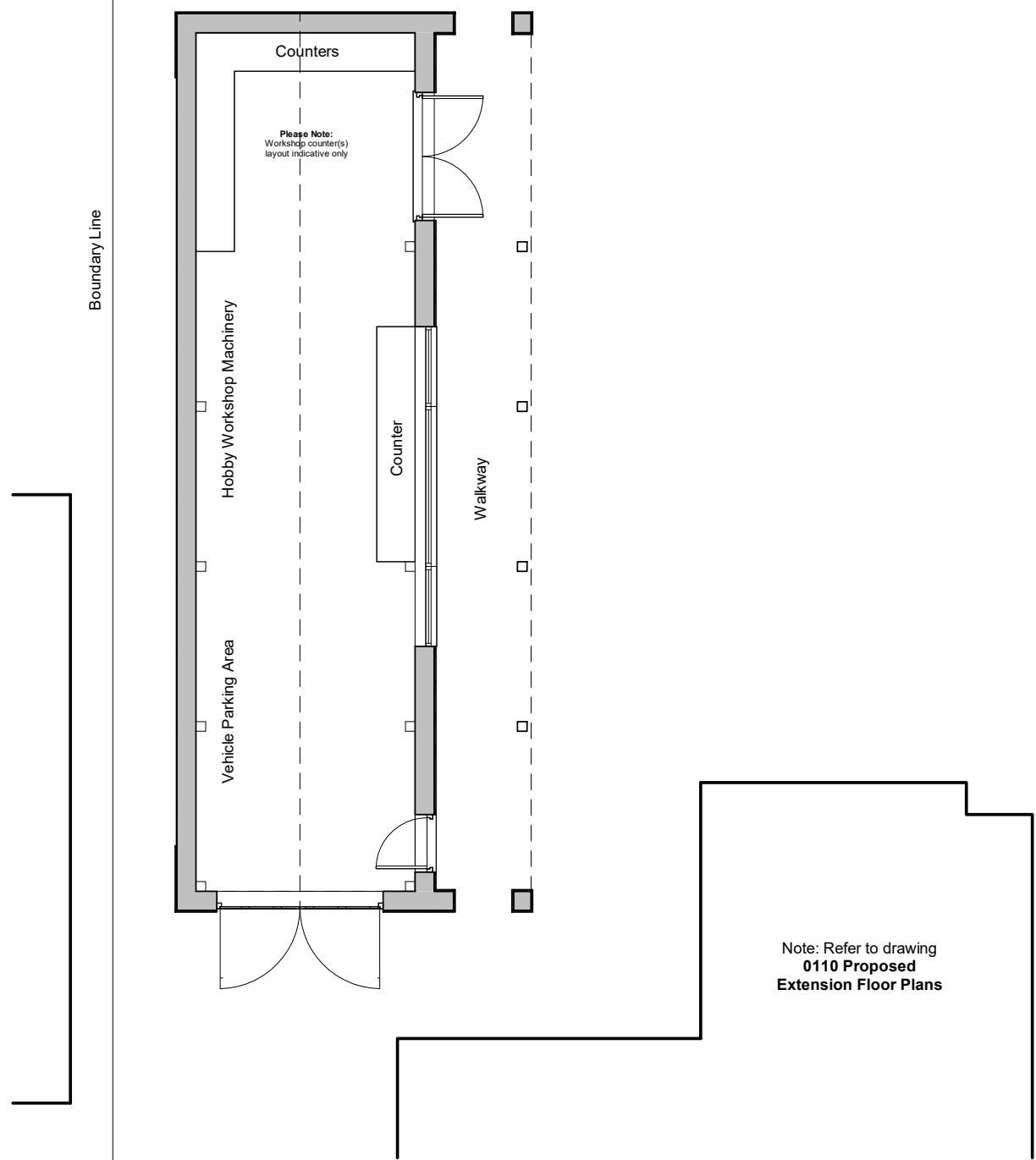
1 Ground Floor FFL 1 : 100
