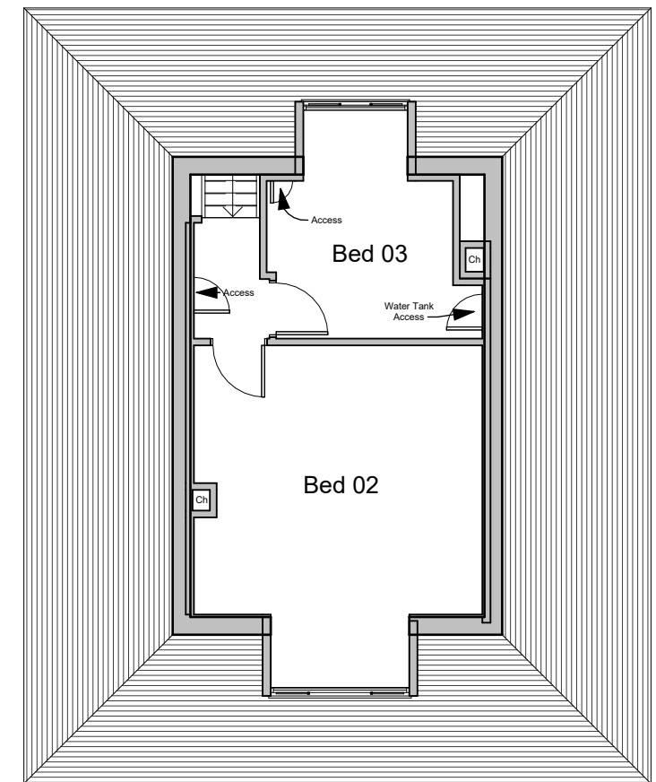
2 First Floor FFL 1 : 100
