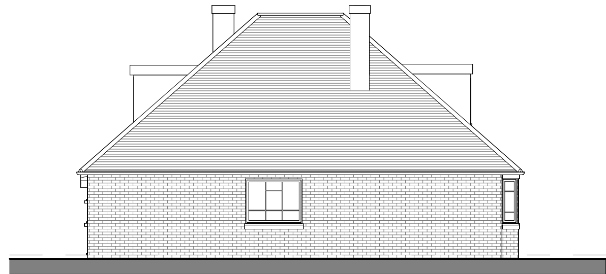
4 North Elevation 1 : 100
