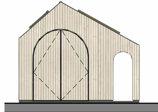
2 West Elevation 1 : 100
