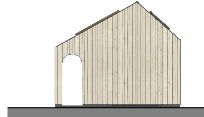
3 East Elevation 1 : 100
