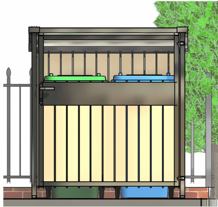
2 FRONT Scale 1:20
