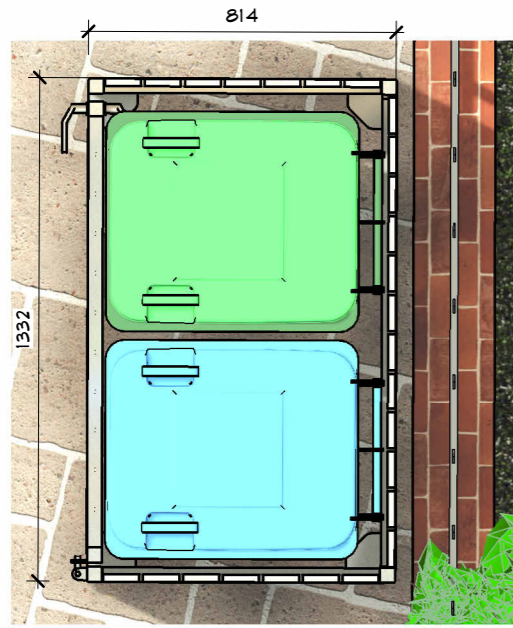
1 BIN SHED Scale 1:20
